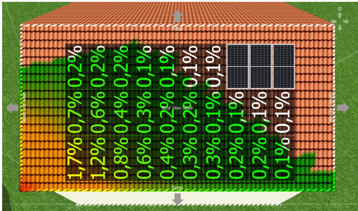
Figure 18: Shading on a yearly basis from a tree with PV modules positioned vertically
