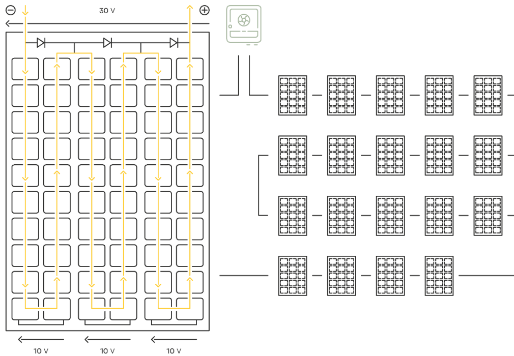
Figure 4: PV system with 20 standard PV modules without shading
