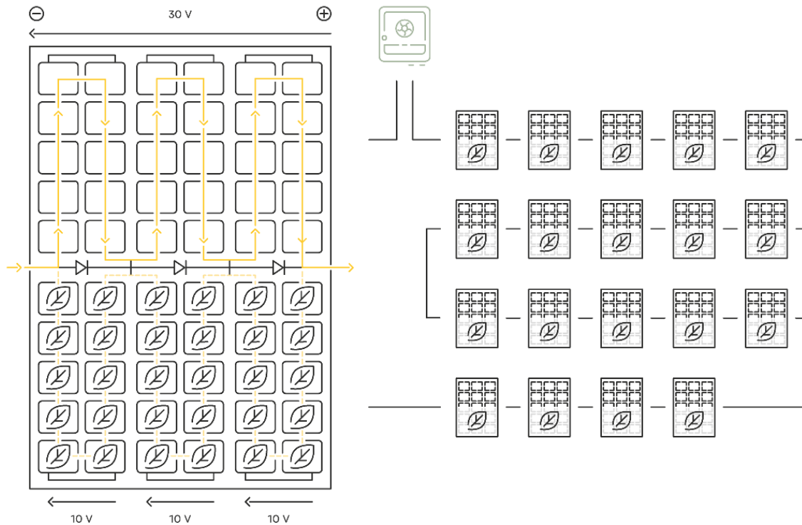
Figure 6: PV system with 20 half-cut PV modules with equal shading.
