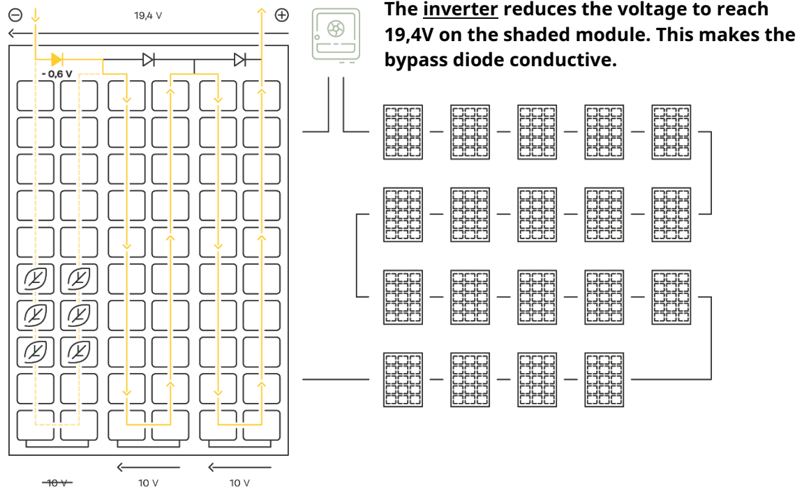
Figure 5: PV system with 20 standard PV modules with shading
