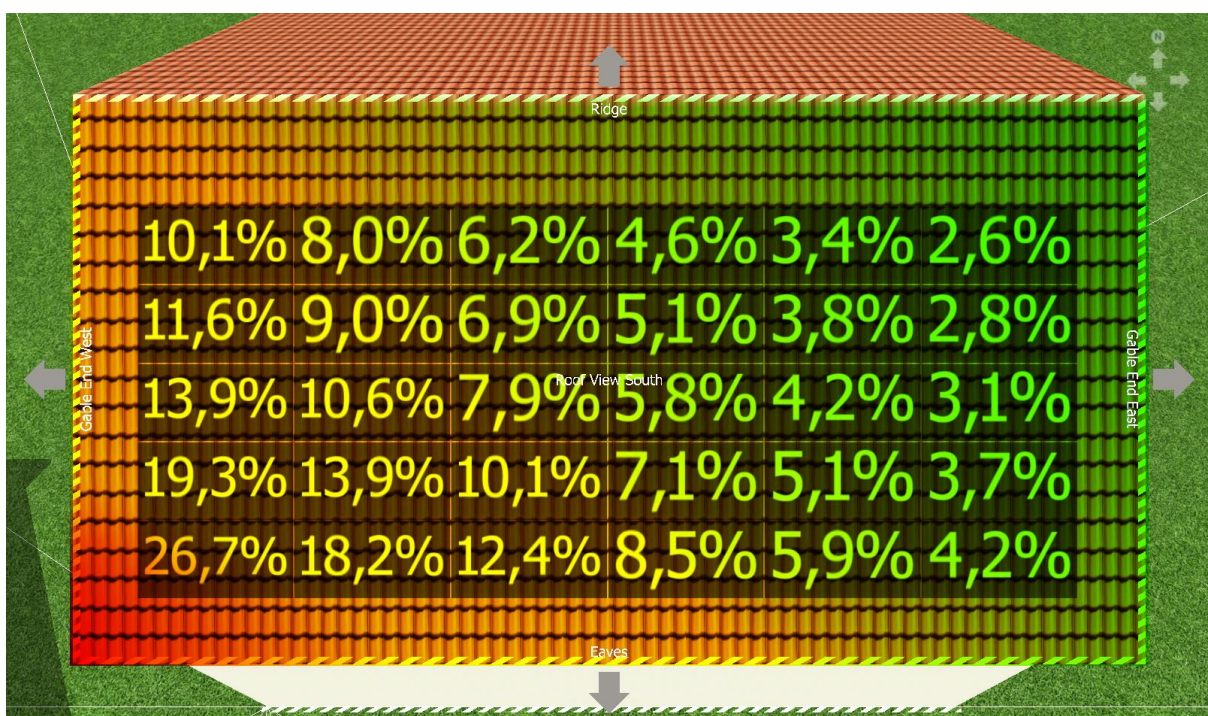
Figure 20: Shading on a yearly basis from another house with PV modules positioned horizontally
