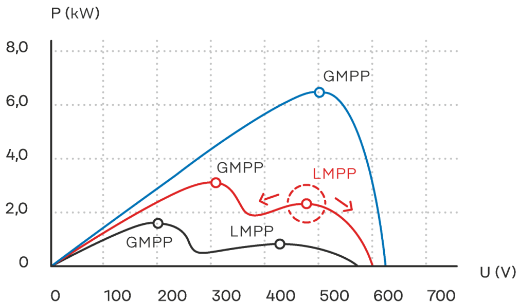
Figure 9: P-V curve with presented GMPP and LMPP
