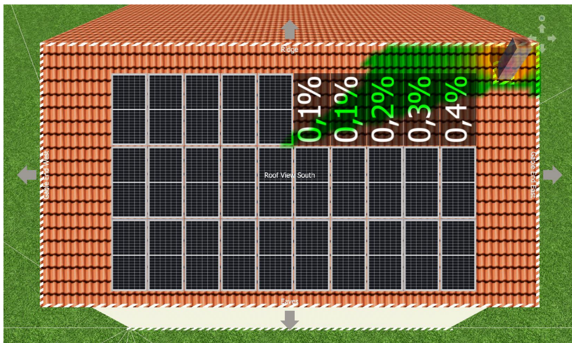
Figure 12: Shading on a yearly basis from a chimney with PV modules positioned vertically
