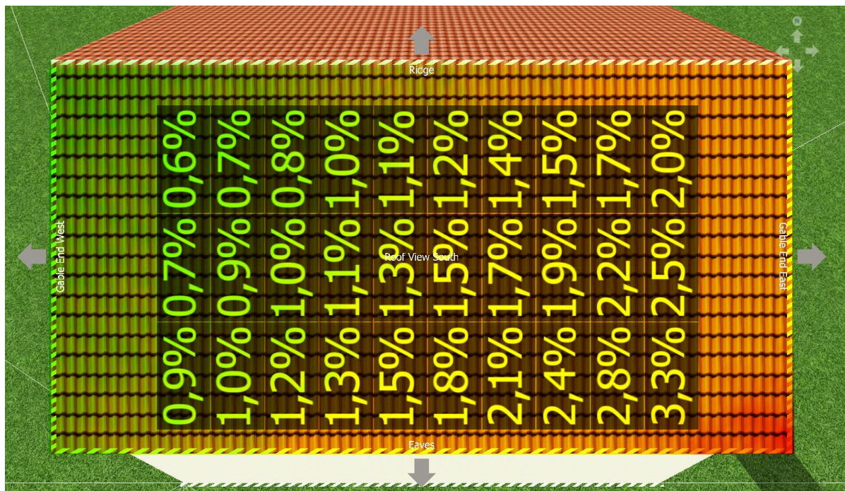
Figure 26: Shading on a yearly basis from another house with PV modules positioned vertically
