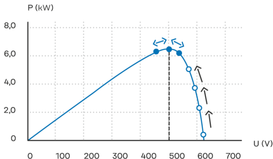
Figure 8: Hill climbing MPP tracking algorithm
