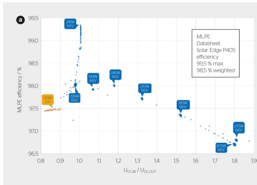
Figure 10: DC/DC optimizer efficiency curve
