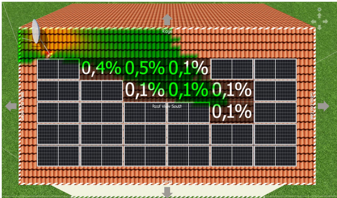
Figure 13: Shading from an antenna with PV modules positioned horizontally
