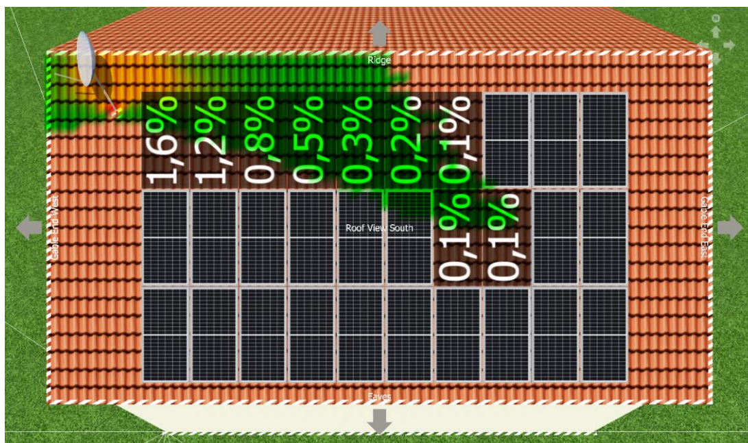
Figure 14: Shading from an antenna with PV modules positioned vertically
