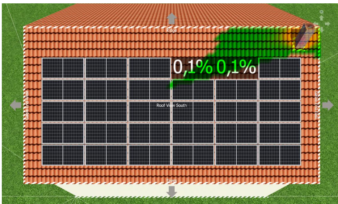
Figure 11: Shading on a yearly basis from a chimney, with PV modules positioned horizontally
