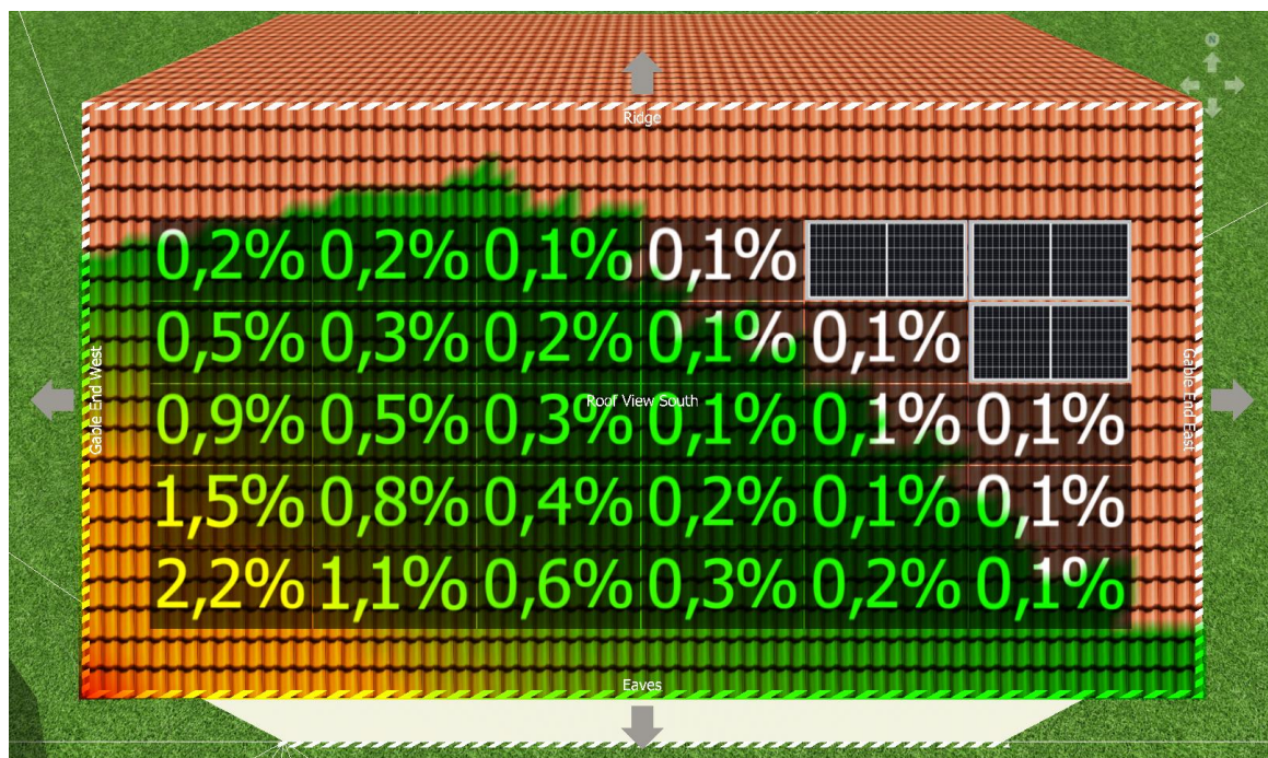
Figure 16: Shading on a yearly basis from a tree with PV modules positioned horizontally
