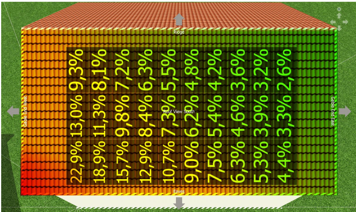
Figure 22: Shading on a yearly basis from another house with PV modules positioned vertically
