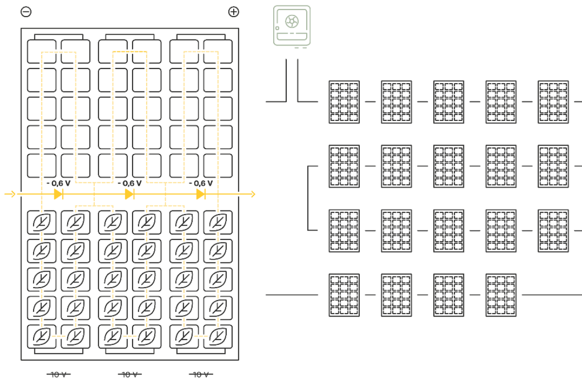
Figure 7: PV system with 20 half-cut PV modules with uneven shading.
